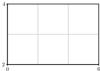
Figure 11.1.1. Rectangular domain R with subrectangles.
